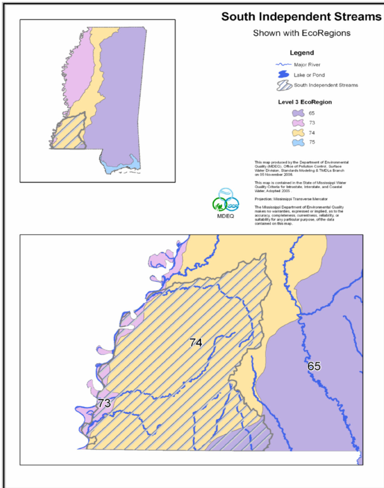
Figure 4. South Independent Streams Basin with Level III Ecoregions
