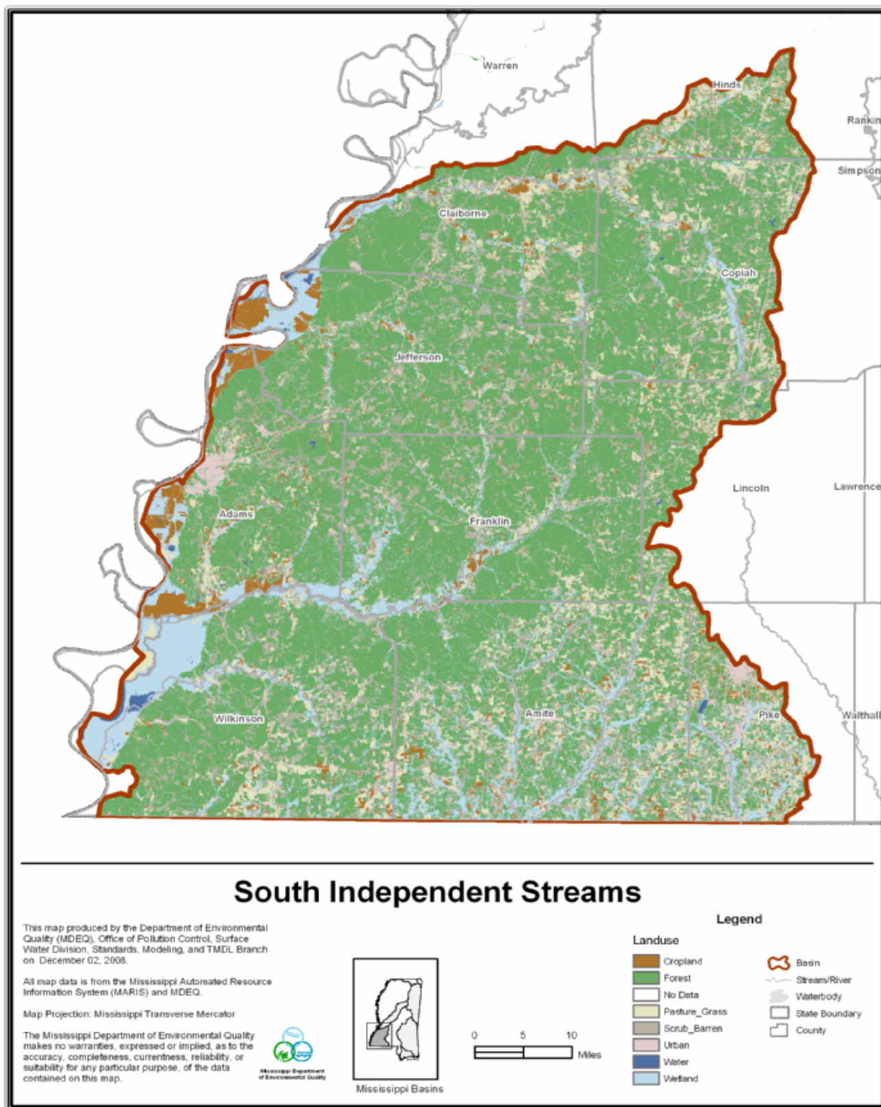
Figure 2. South Independent Streams Basin Landuse Distribution
