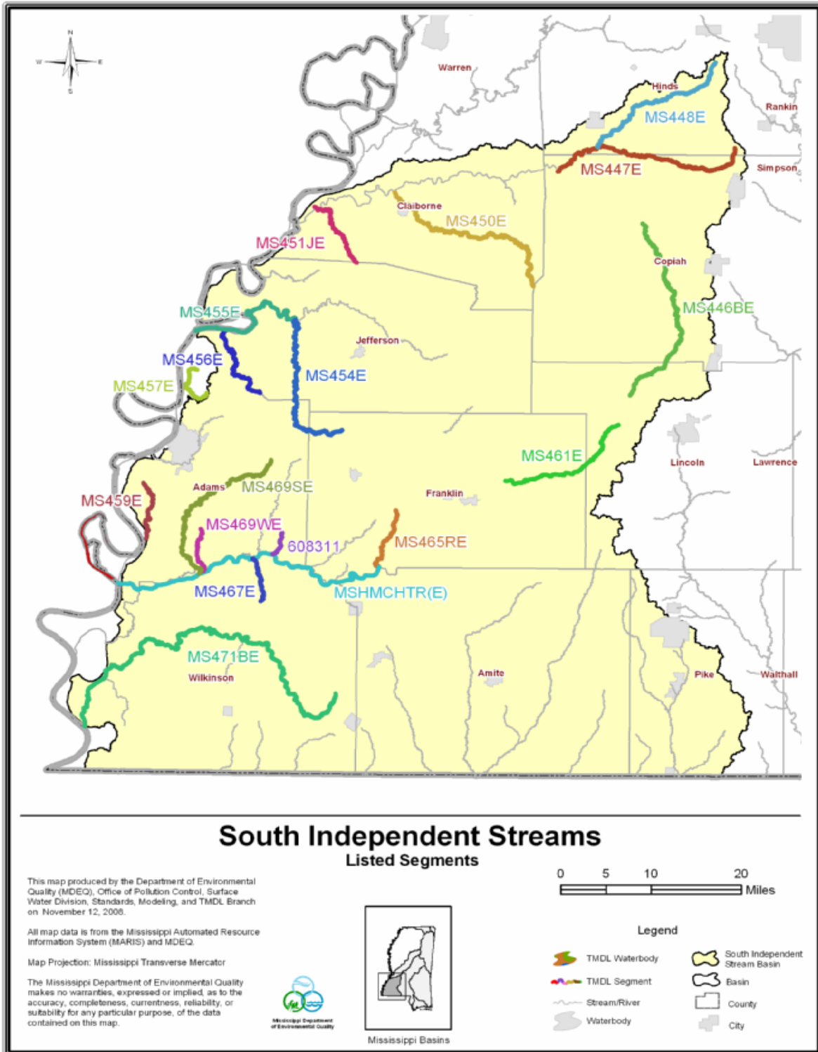
Figure 1. Location of South Independent Streams Basin §303(d) Listed Segments
